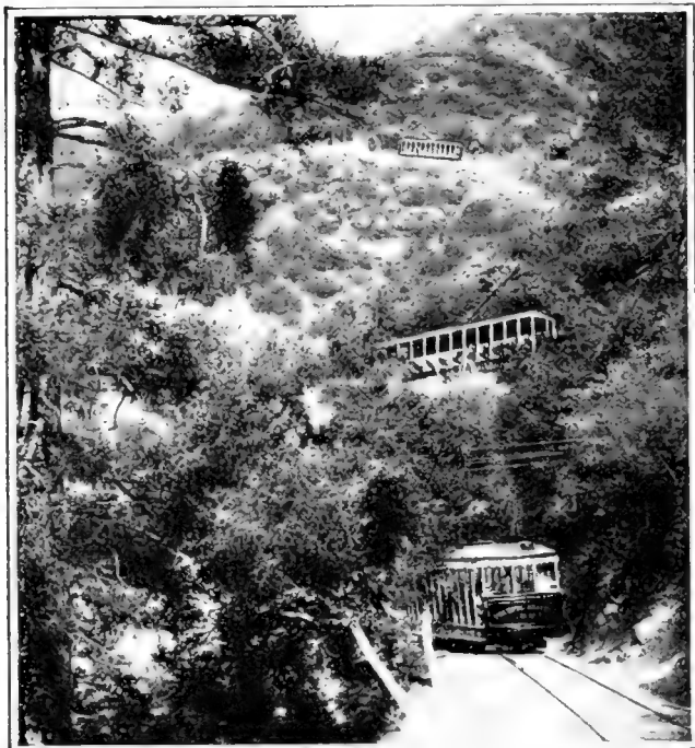
Three levels of track are visible in the zig-zag course up the precipitous mountain side
